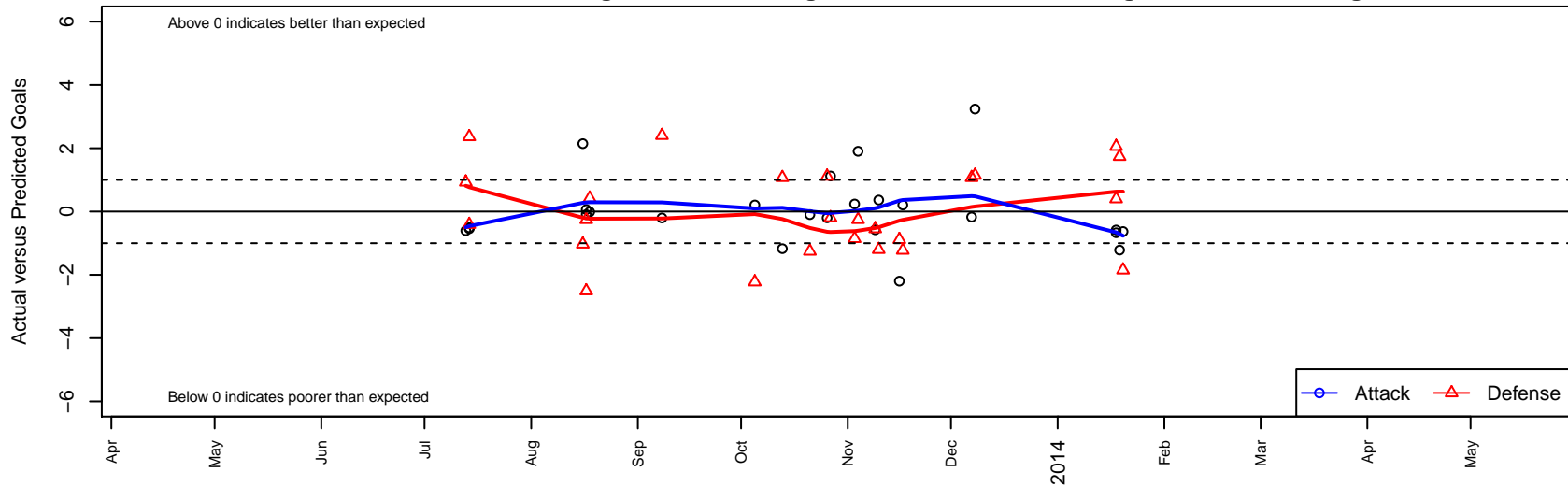
SSC Shadow A B97 Dots are actual minus expected GF (blue circles) and GA (red triangles). Blue line is smoothed change in attack strength. Red is smoothed change in defense strength.
